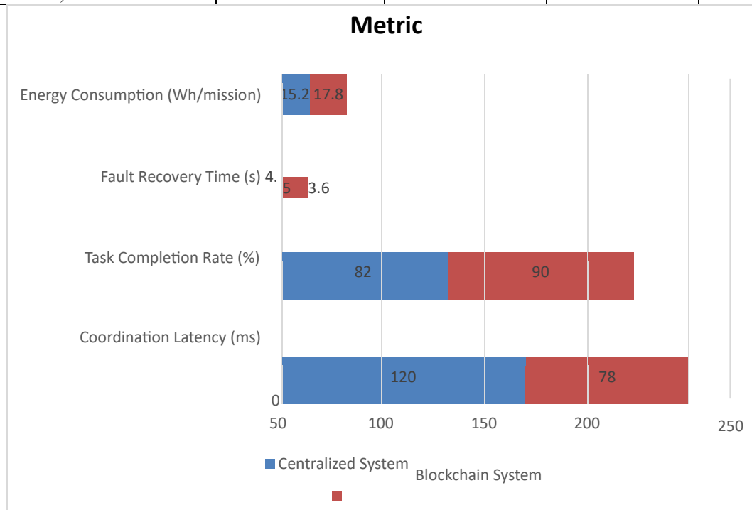
Figure-3. Comparative Performance Metrics across 100 Runs in a 10-Robot Deployment
