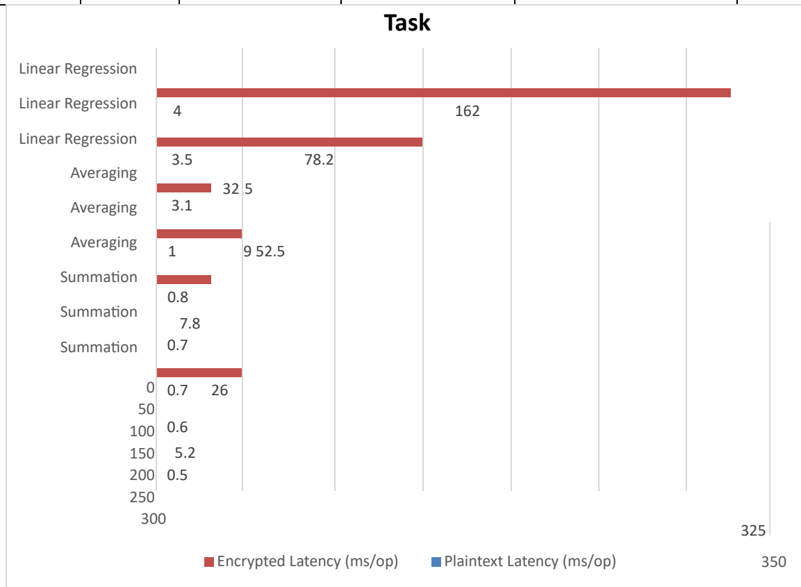
Figure-3. Performance Comparison between Plaintext and Homomorphic Encryption Workloads
