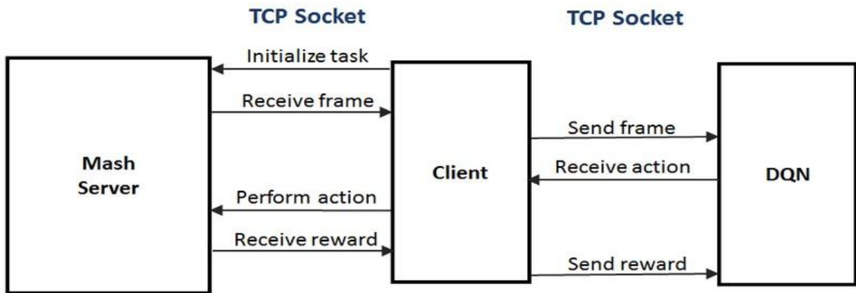
Fig.1 Reinforcement Learning, Source:1
